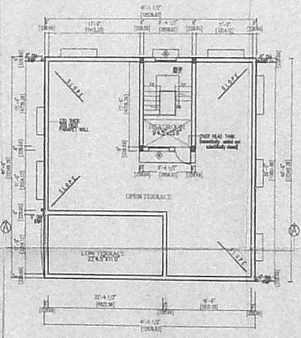
TOPO PLAN
